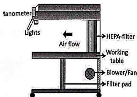
Horizontal Laminar Flow Cabinet
