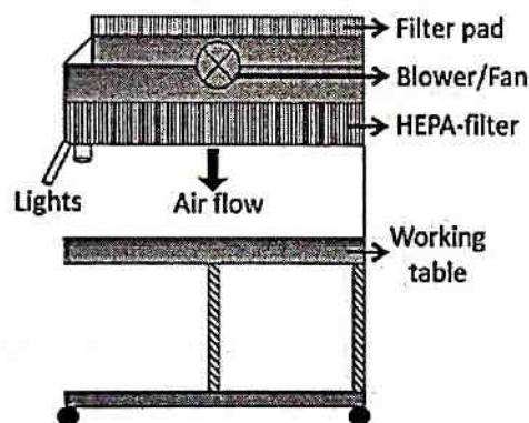
Vertical Laminar Flow Cabinet
