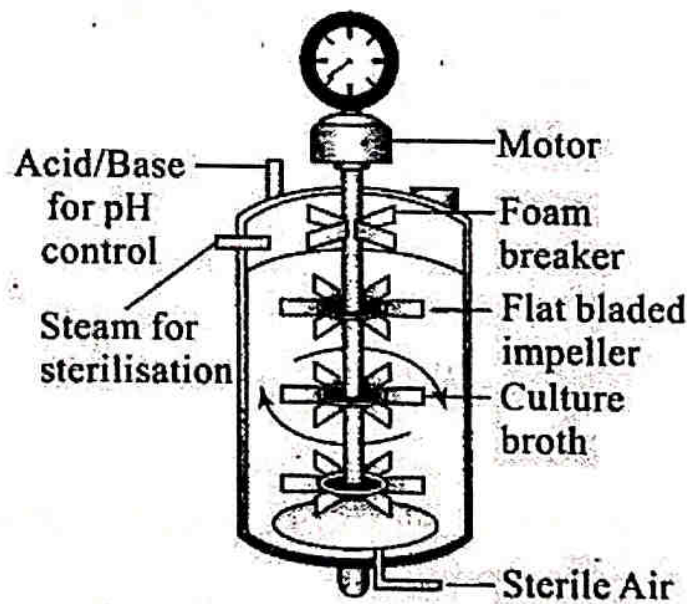
Simple stirred-tank bioreactor
